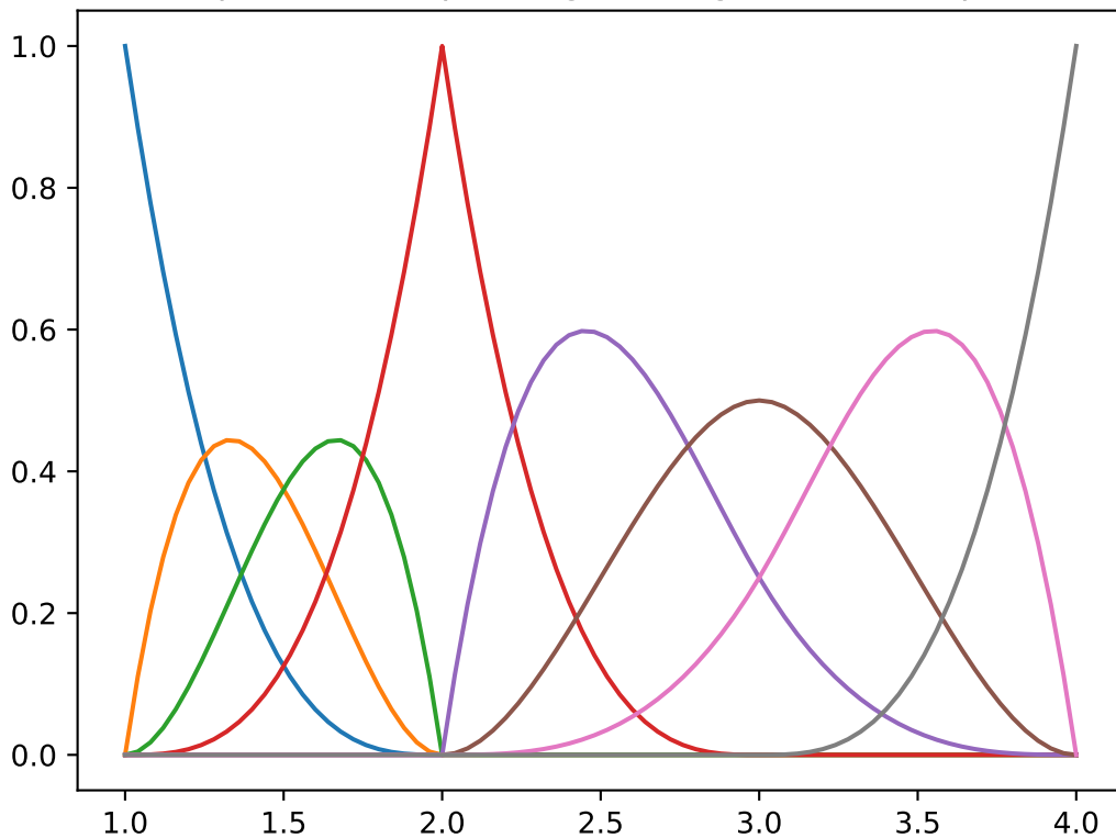
8 B-Splines corresponding to the given knot sequence
