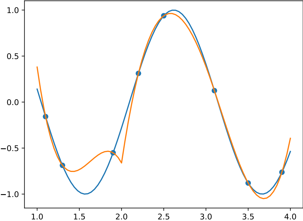
Piecewise polynomial spline approximation of function through data sites
